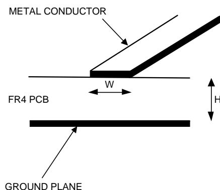
Figure 95. Microstrip Configuration
