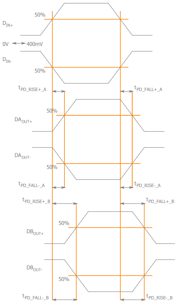
Figure 3. Rise / Fall Propagation Delay &amp; Skew
