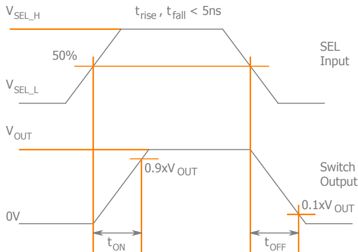
Figure 1. t_{ON}, t_{OFF}
