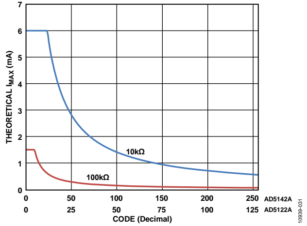
Figure 31. Theoretical Maximum Current vs. Code
