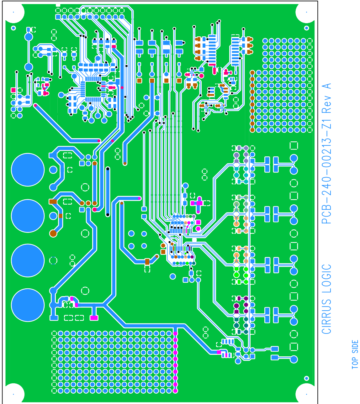
Figure 24. Top Routing
