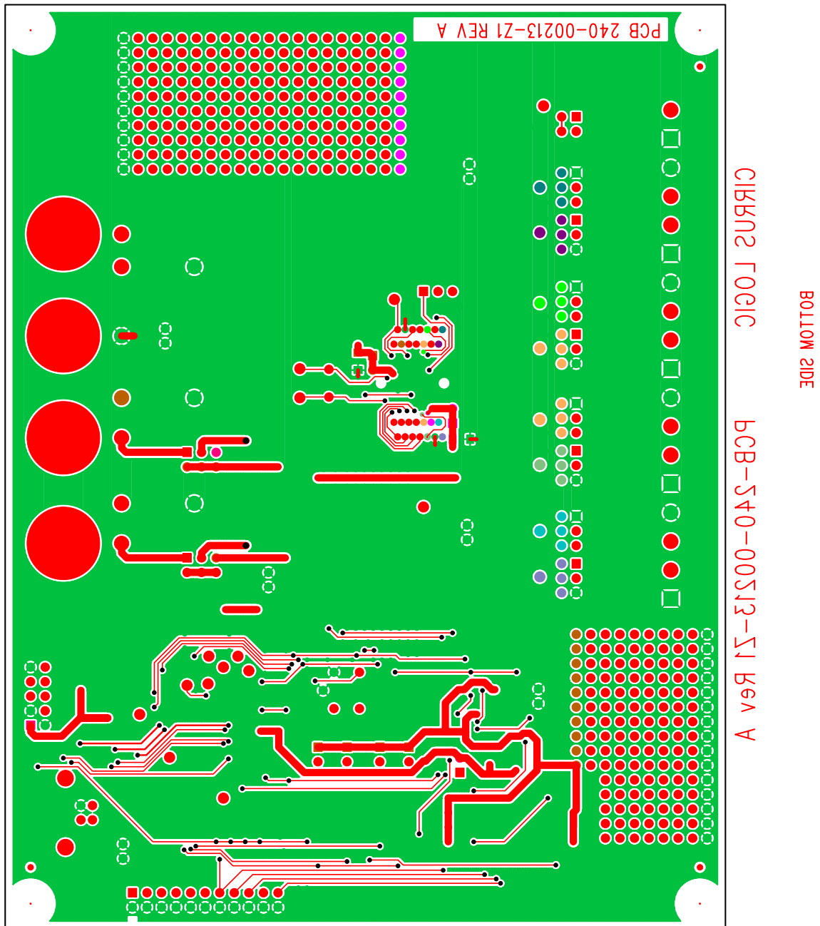
Figure 25. Bottom Routing
