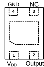
DFN1216-4
