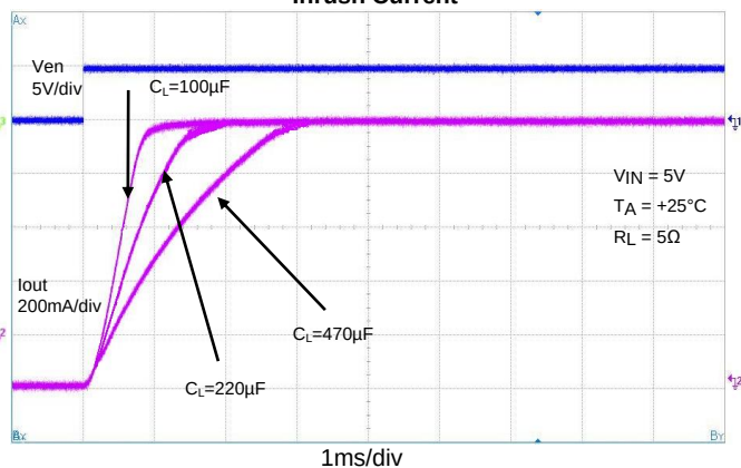
Inrush Current
