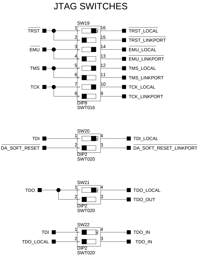
MULTI PROCESSOR JTAG SETTINGS VIA HP-USB EMUALTOR USING TWO OR MORE EZ-BOARDS (LINK PORT CABLES REQUIRED FOR MORE THAN TWO BOARDS)
