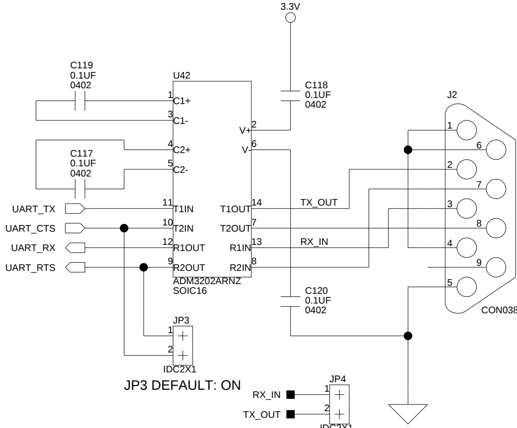
LOOPBACK HEADER FOR TESTING PURPOSES ONLY JP4 DEFAULT: OFF
