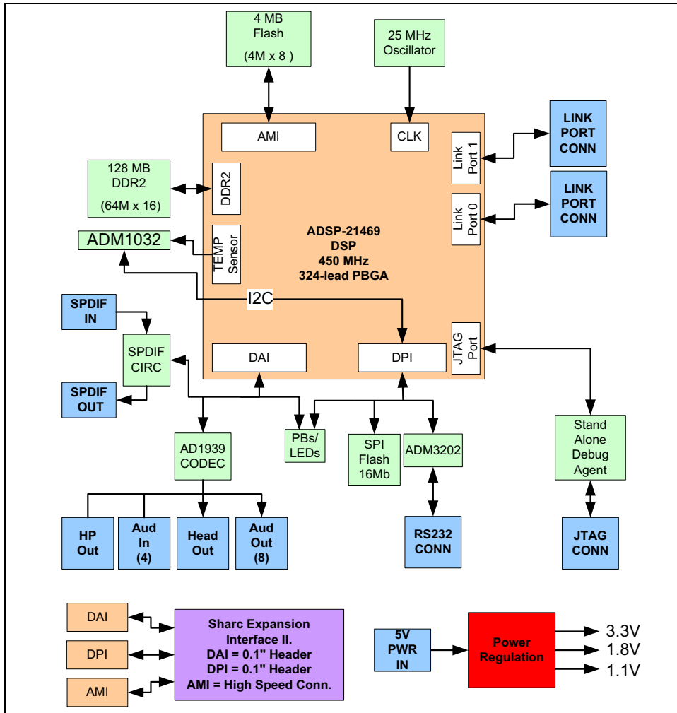
Figure 2-1. System Architecture
