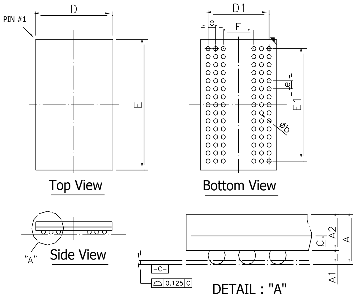
Figure 43. 90 ball TFBGA 8x13x1.2mm(max.) Outline Drawing Information
