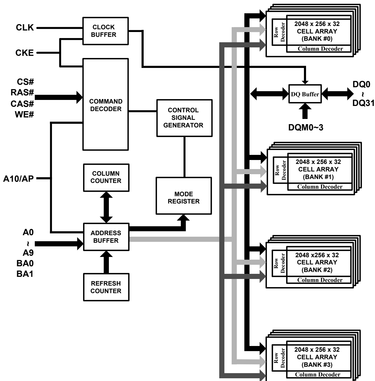
Figure 2. Block Diagram
