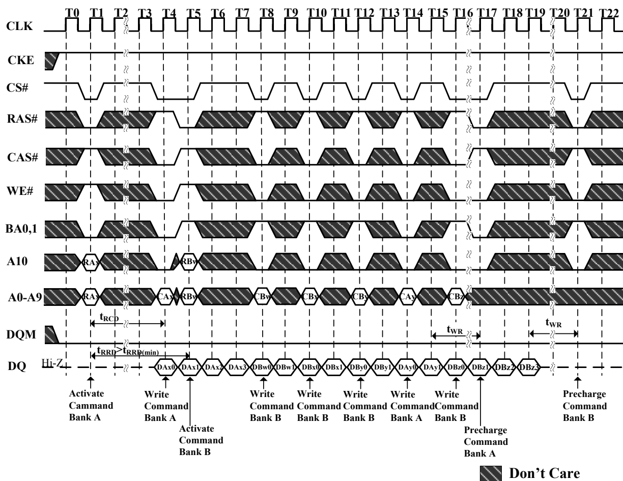
Figure 33. Interleaved Column Write Cycle (Burst Length=4)
