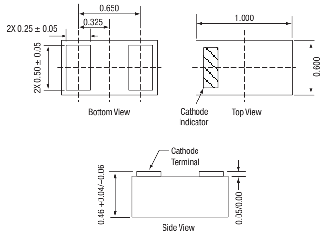
Package Dimensions
