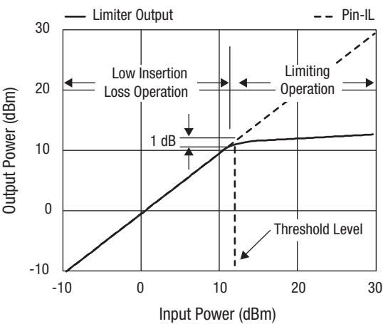
Output Power vs. Input Power for a Single Stage Limiter
