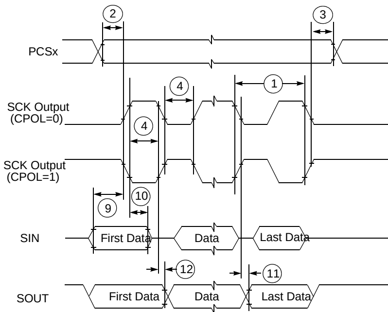
Figure 33. DSPI classic SPI timing—master, CPHA = 0
