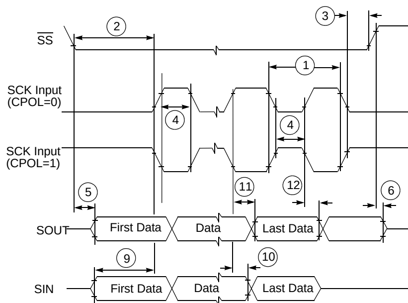
Figure 39. DSPI modified transfer format timing—slave, CPHA = 0
