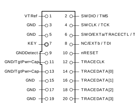
FIGURE 41 The Cortex20 pinout of the Cortex side of the ADA-ETM-SWD20 probe. Top view.
