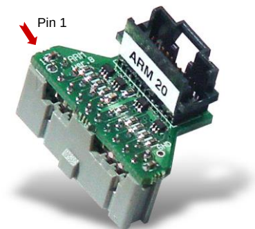
FIGURE 1 The 20-pin JTAG ADA-JET-ARM20 probe for ARM.
