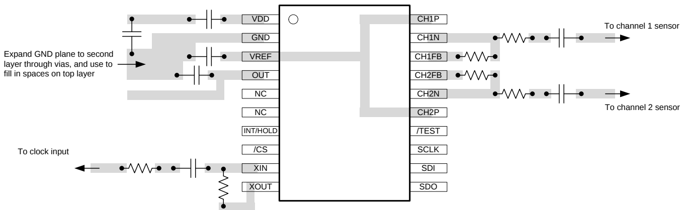
Figure 7. PCB Layout Example
