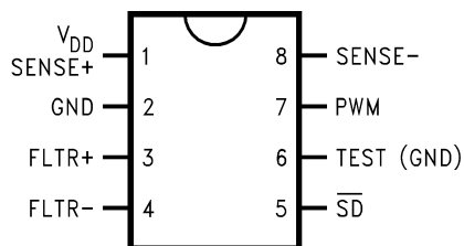
Figure 1. Top View LM3822 for High-Side Sensing
