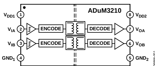
Figure 1. ADuM3210
