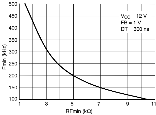
Figure 36. Minimum Switching Frequency Resistor Selection ( F_{min} = 100\text{ kHz} to 500\text{ kHz} )
