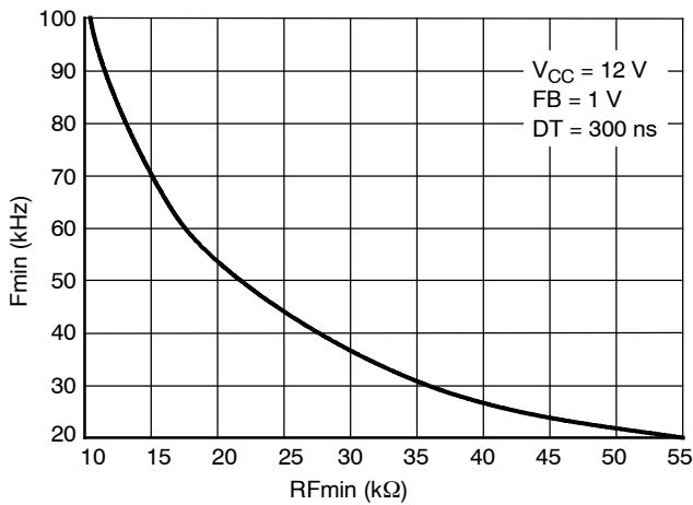
Figure 37. Minimum Switching Frequency Resistor Selection ( F_{min} = 20\text{ kHz} to 100\text{ kHz} )
