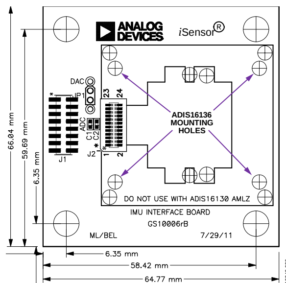
Figure 22. Physical Diagram for the ADIS16IMU1/PCBZ
