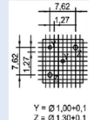
Drilling diagram:
