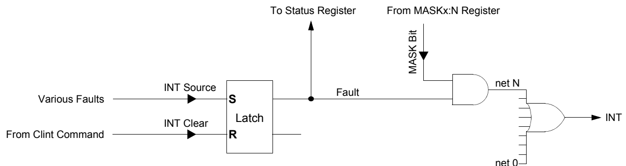
Figure 18. Interrupt Handling
