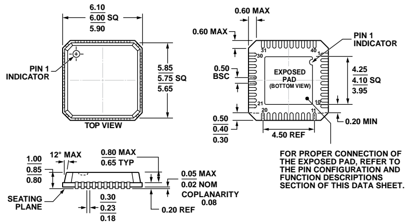
Figure 49. 40-Lead Lead Frame Chip Scale Package [LFCSP_VQ] 6 mm × 6 mm Body, Very Thin Quad (CP-40-1)
