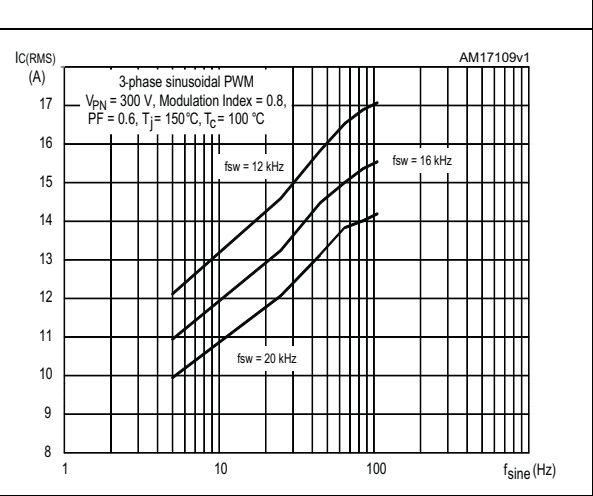
Figure 4. Maximum I_{C(RMS)} current vs. f_{sine} (1)
