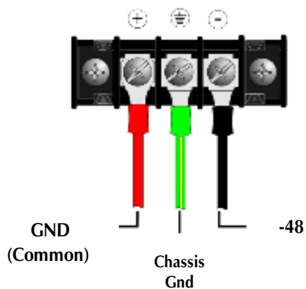
Terminal Block
