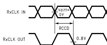
Figure 15. DS90CF562 (Receiver) Clock In to Clock Out Delay
