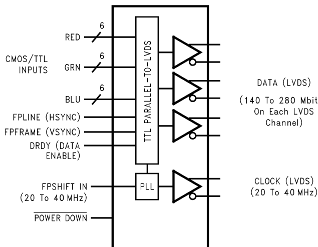
Figure 1. DS90CF561 See Package Number DGG0048A
