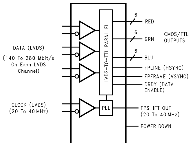
Figure 2. DS90CF562 See Package Number DGG0048A
