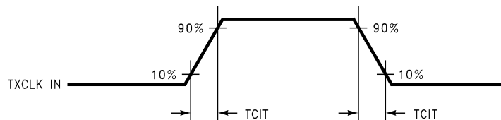
Figure 10. DS90CF561 (Transmitter) Input Clock Transition Time
