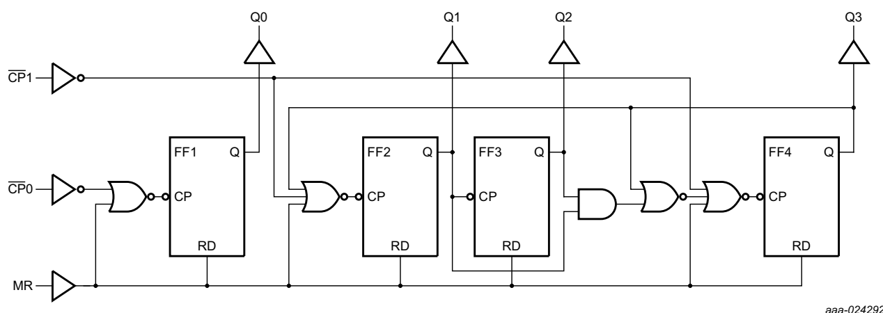
Fig 2. Logic diagram (one counter)
