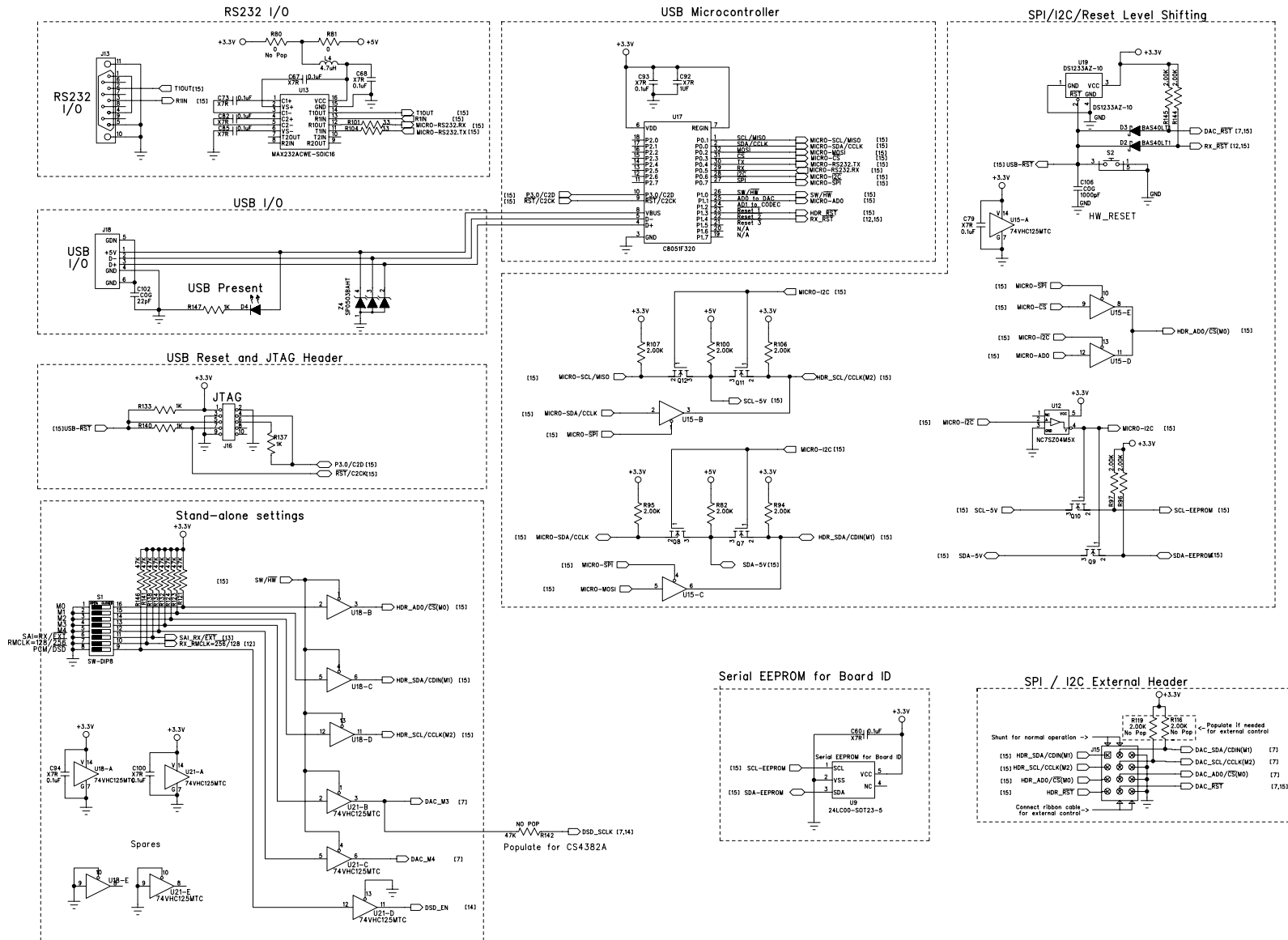
Figure 52. Control Input
