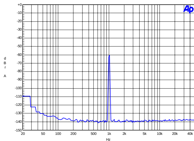
Figure 19. FFT (96 kHz, -60 dB Wideband)
