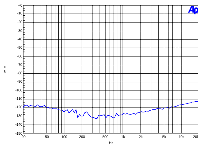
Figure 39. 192 kHz, Crosstalk
