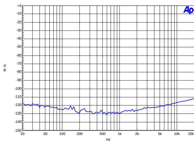
Figure 11. 48 kHz, Crosstalk
