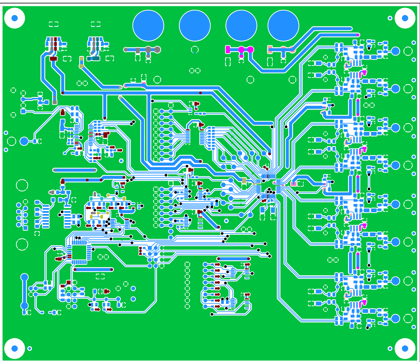
Figure 55. Top Side
