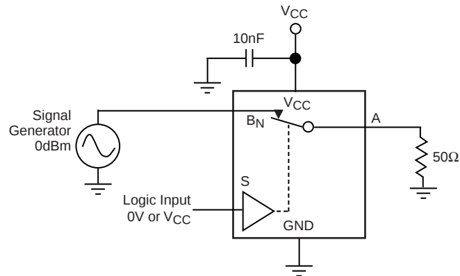
Figure 9. Bandwidth
