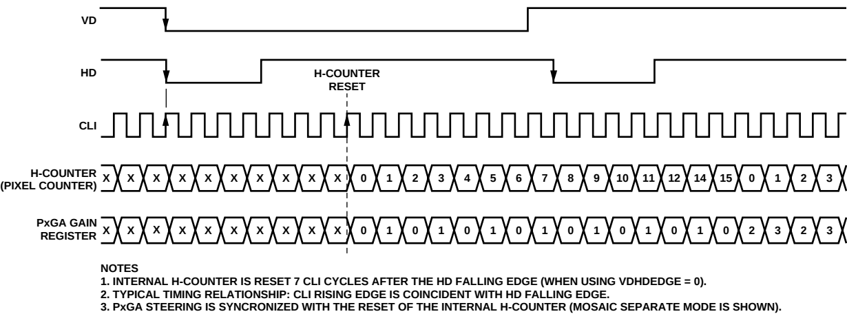
Figure 26. H-Counter Synchronization
