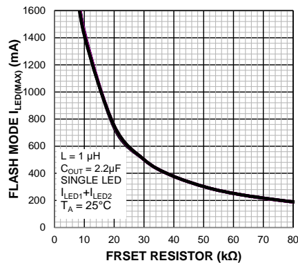
Flash Mode I_{\text{LED(MAX)}} (Single LED) vs. FRSET Resistor
