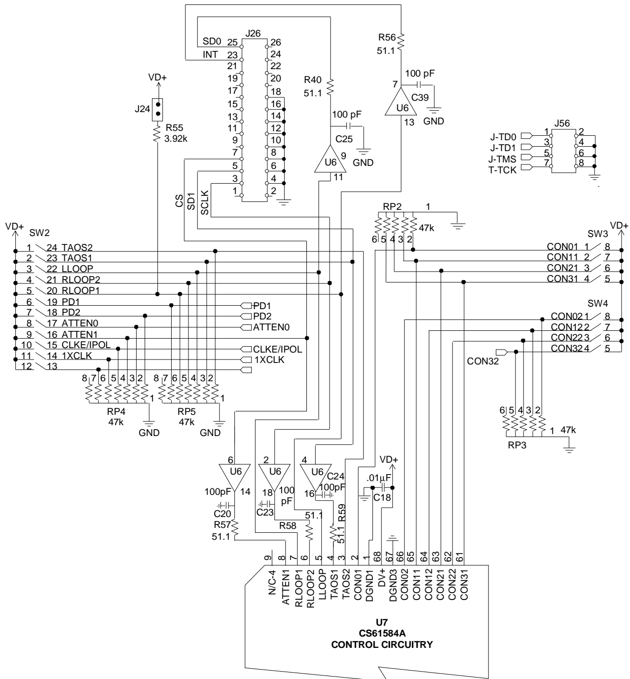
Figure 3. Control Circuitry
