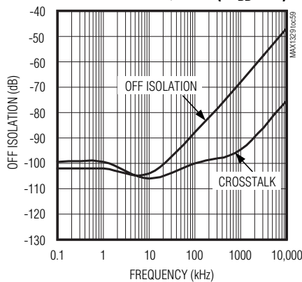
ANALOG SWITCH CROSSTALK AND OFF ISOLATION vs. FREQUENCY ( V_{DD} = 3V )
