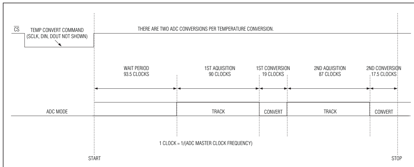
Figure 22. Temperature-Conversion Timing
