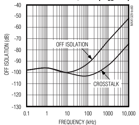
ANALOG SWITCH CROSSTALK AND OFF ISOLATION vs. FREQUENCY ( V_{DD} = 5V )
