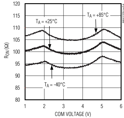
ANALOG SWITCH ON-RESISTANCE vs. COM VOLTAGE ( V_{DD} = 5V )
