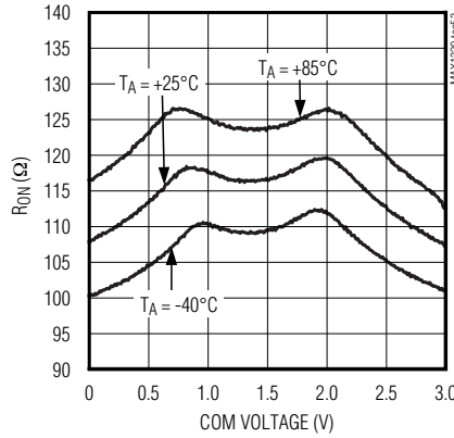
ANALOG SWITCH ON-RESISTANCE vs. COM VOLTAGE ( V_{DD} = 3V )
