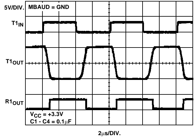
FIGURE 6. LOOPBACK TEST AT 250kbps ( C_L = 1000\text{pF} )
