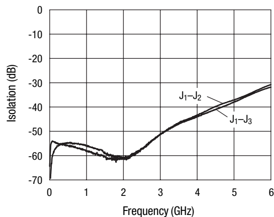
Isolation, 25 °C
