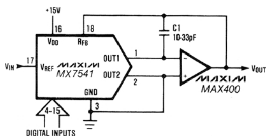
Unipolar Operation
