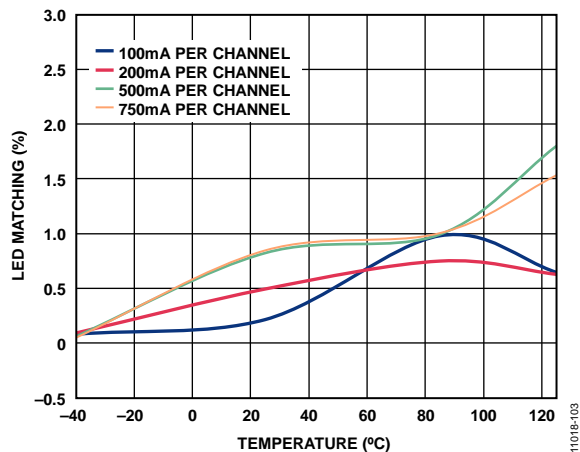
Figure 15. LED Matching vs. Temperature
