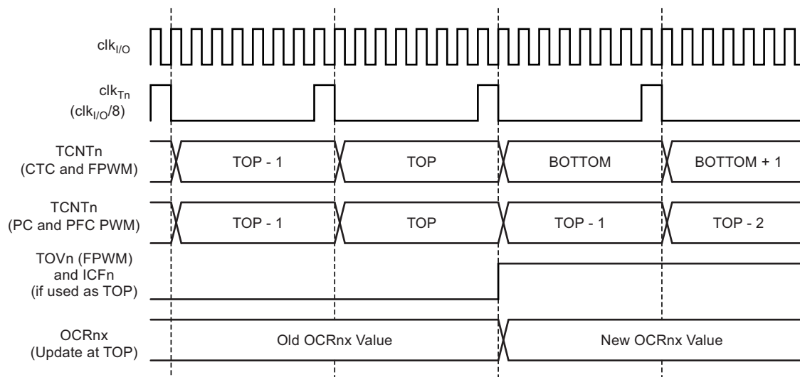
Figure 5-52. Timer/Counter Timing Diagram, with Prescaler ( f_{\text{clk\_I/O}}/8 )
