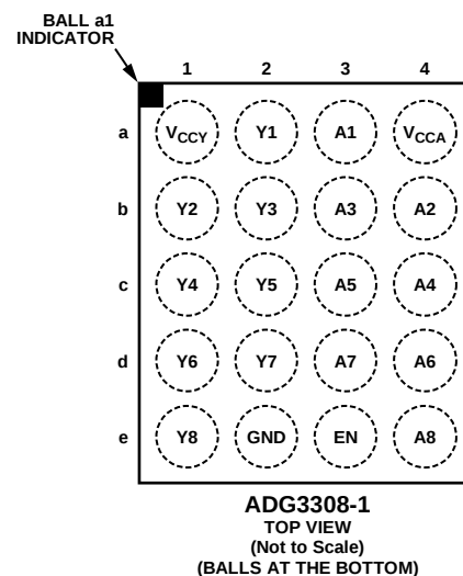
Figure 4. 20-Ball WLCSP
