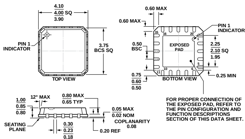
Figure 43. 20-Lead Lead Frame Chip Scale Package [LFCSP_VQ] 4 mm × 4 mm Body, Very Thin Quad (CP-20-1)
