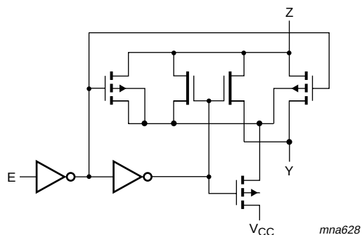
Fig 2. Logic diagram
