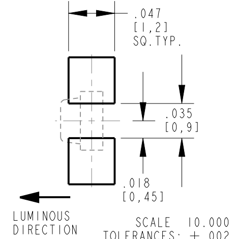
RECOMMENDED SOLDERING PAD LAYOUT
