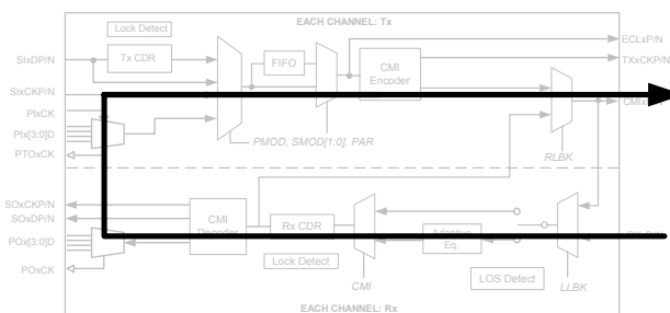
Figure 9: Remote (Digital) Loopback
