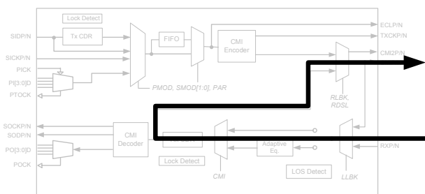
Figure 8: Remote (Analog) Loopback
