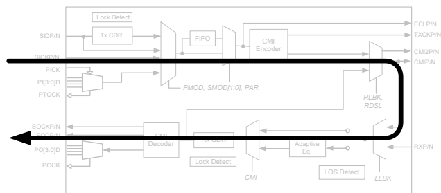
Figure 7: Local (Analog) Loopback
