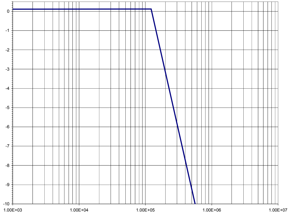
Figure 19: Jitter Transfer
