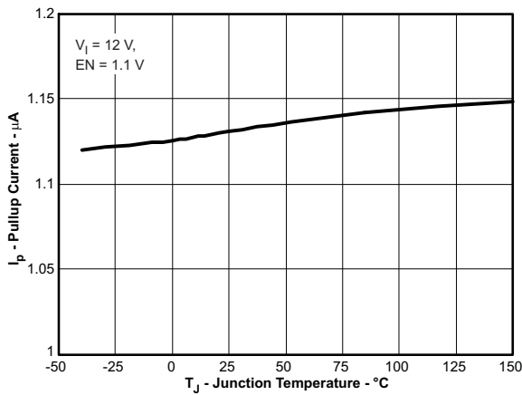
Figure 7. EN Pin Pullup Current vs Temperature
