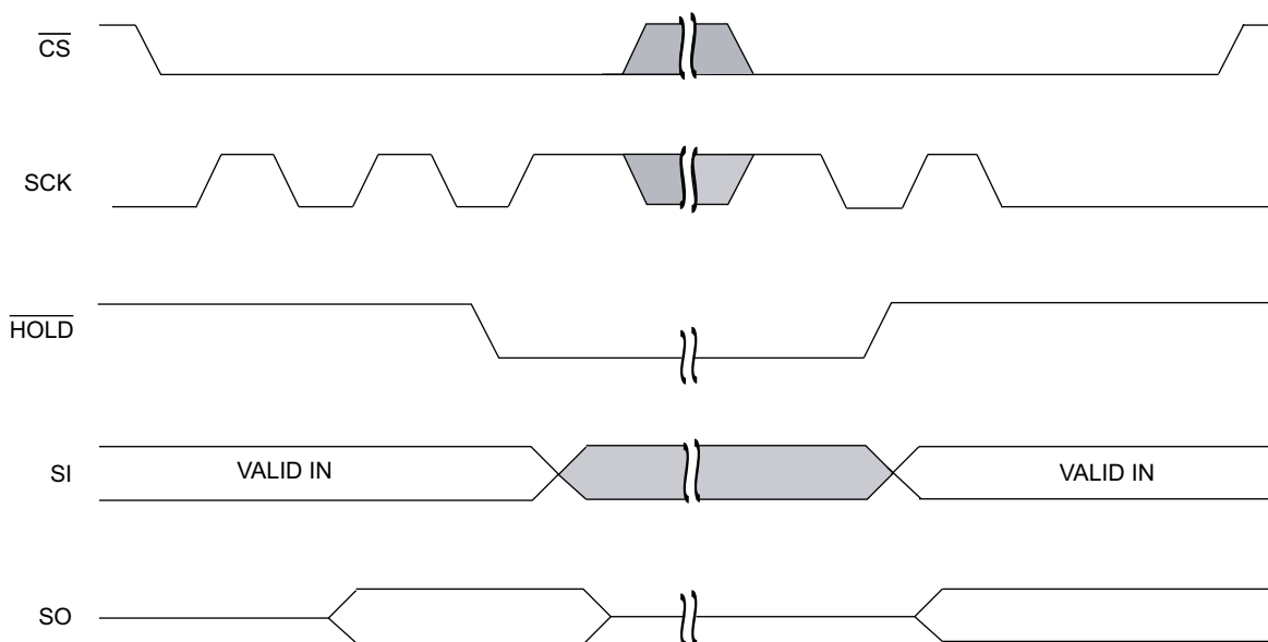
Figure 14. HOLD Operation [2]
