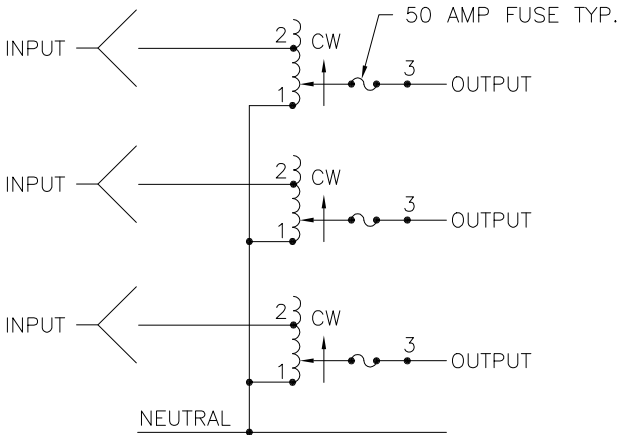
SCHEMATIC
