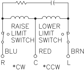
MOTOR CIRCUIT
