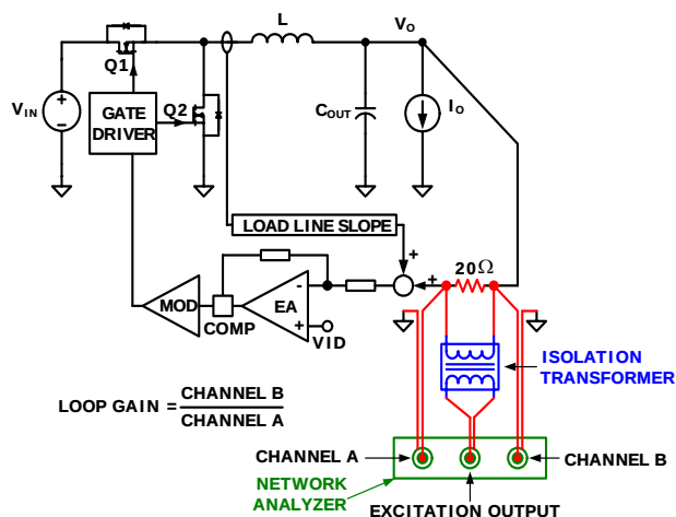
FIGURE 22. LOOP GAIN T2(s) MEASUREMENT SET-UP
