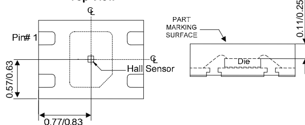
Sensor Location
