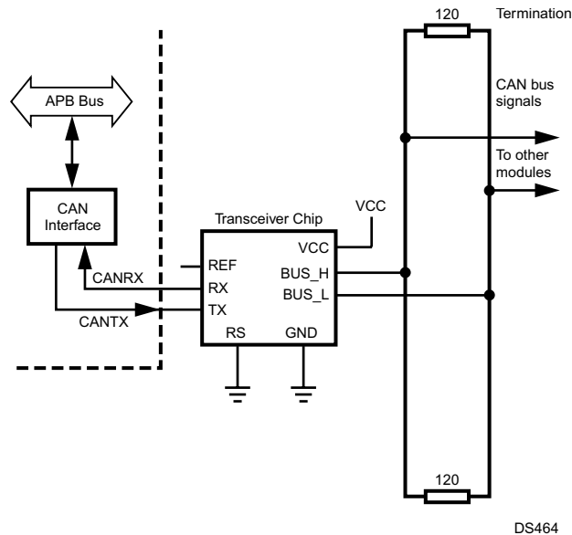
Figure 18-31. External Transceiver
