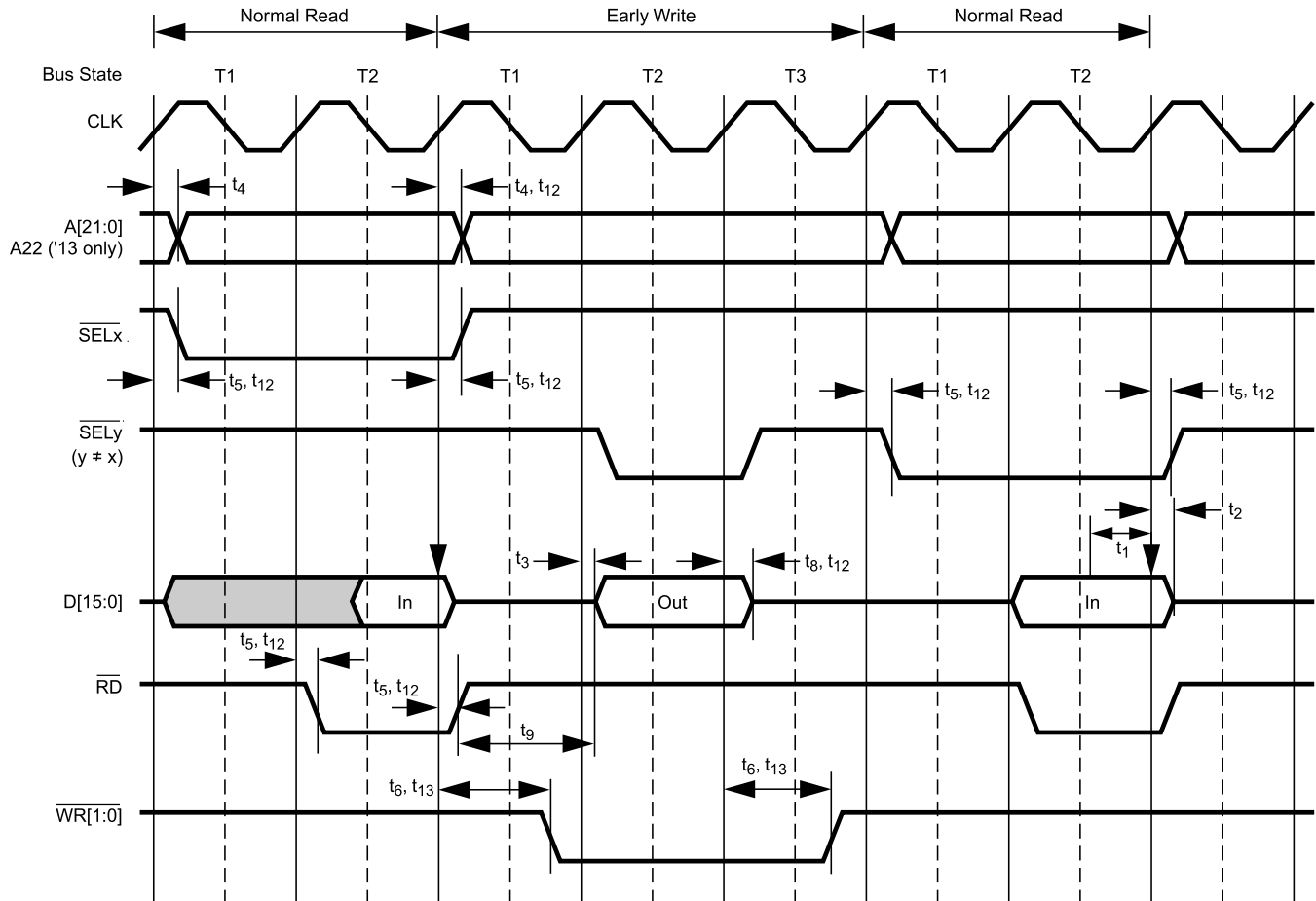
Figure 29-22. Early Write Between Normal Read Cycles (No Wait States)
