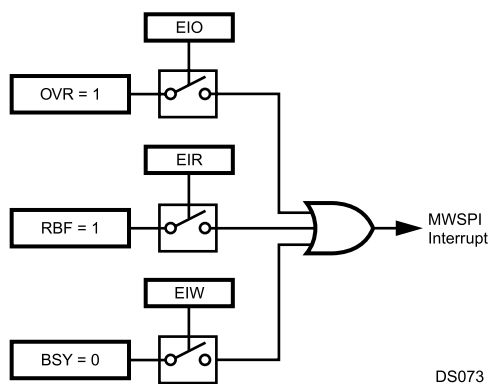
Figure 22-7. MWSPI Interrupts
