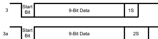
Figure 21-6. 9-bit Data Frame Options
