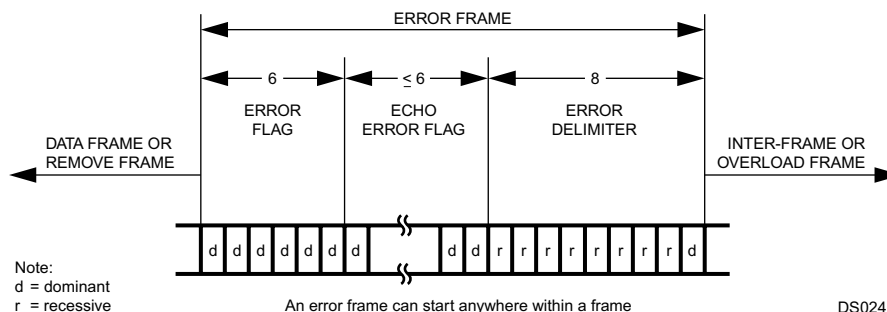
Figure 18-7. Error Frame
