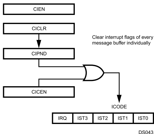
Figure 18-26. Interrupt Management
