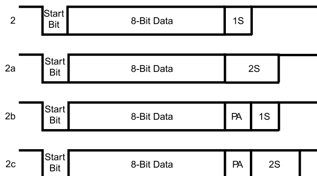
Figure 21-5. 8-Bit Data Frame Options
