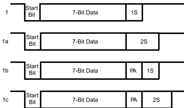
Figure 21-4. 7-Bit Data Frame Options
