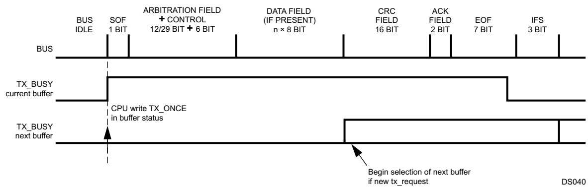
Figure 18-23. Data Transmission
