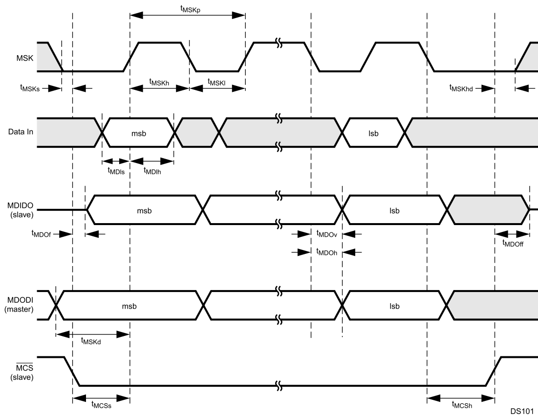
Figure 29-11. Microwire Transaction Timing, Normal Mode, SCIDL = 0
