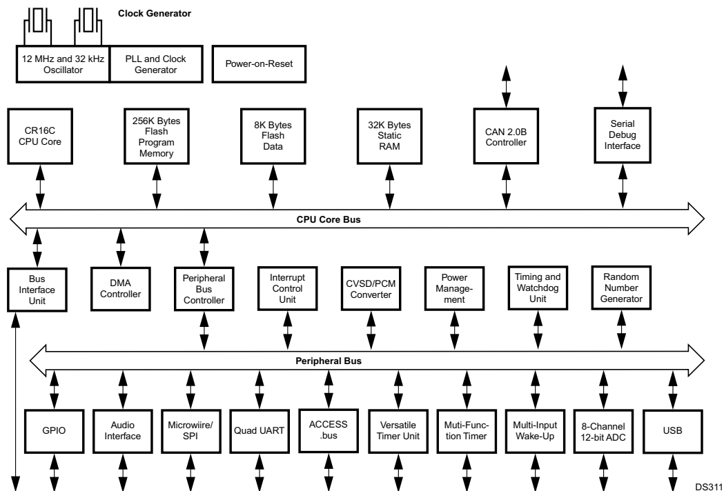
Figure 1-1. Block Diagram
