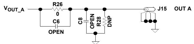
FIGURE 4. OUTPUT STAGE
