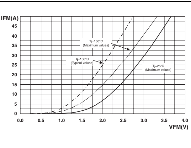
Figure 17. Forward voltage drop versus forward current
