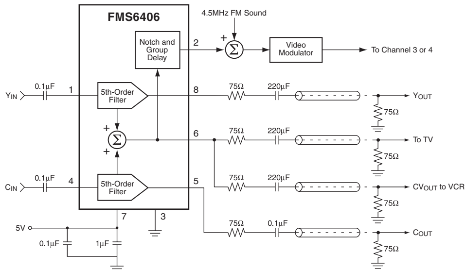
Figure 22. AC-Coupled Application Diagram
