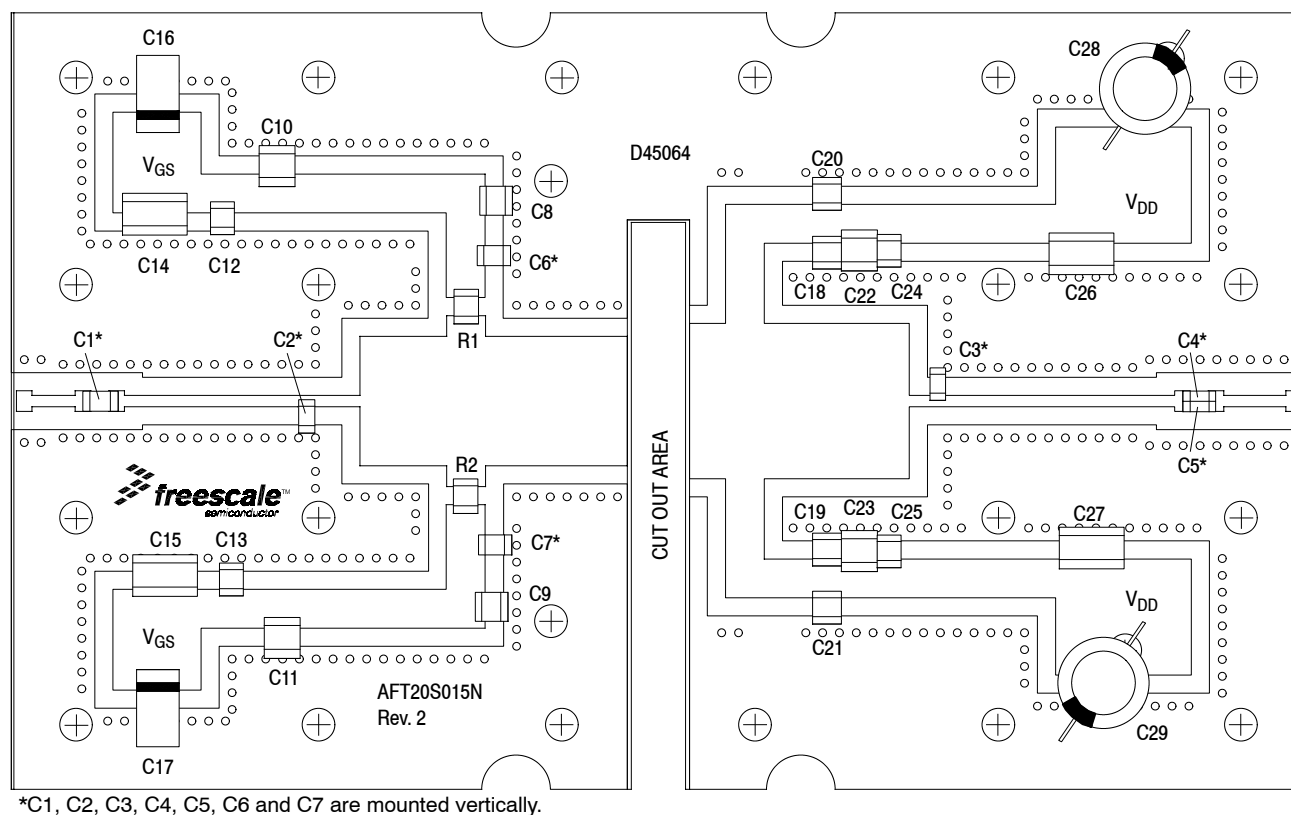
Figure 8. AFT20S015NR1 Test Circuit Component Layout — 1805-1880 MHz
