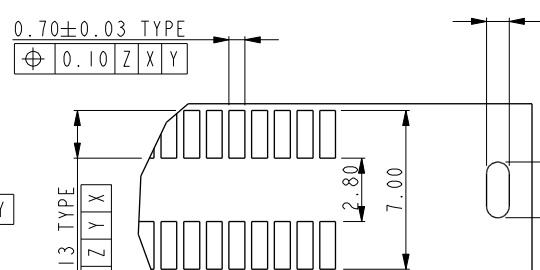
DETAIL E SCALE 3.000 For paste-in-hole applications. Can be used to solder clips during reflow operation.
