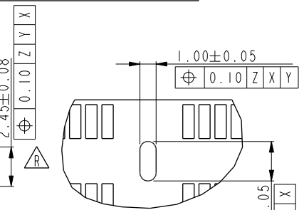
DETAIL D SCALE 3.000 Center forklock type
