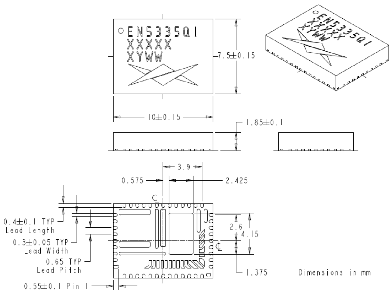
Figure 7. Package Dimensions
